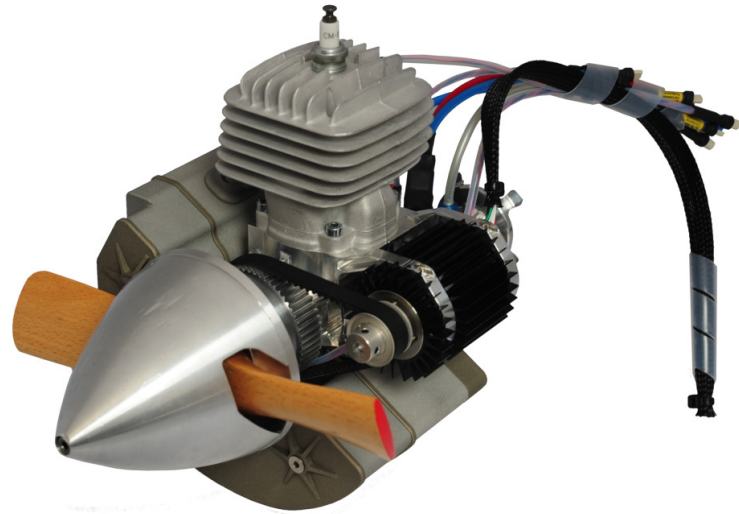
B29i-AXS Engine (2.25kg / 5lb)
