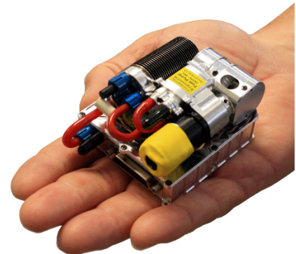
Integrated ECU, Fuel Pump & Accumulator (175g / .39lb)
