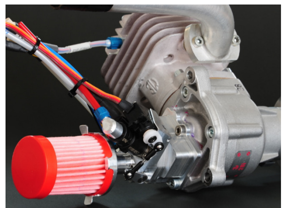
Induction Assembly (123g / .27lb)
